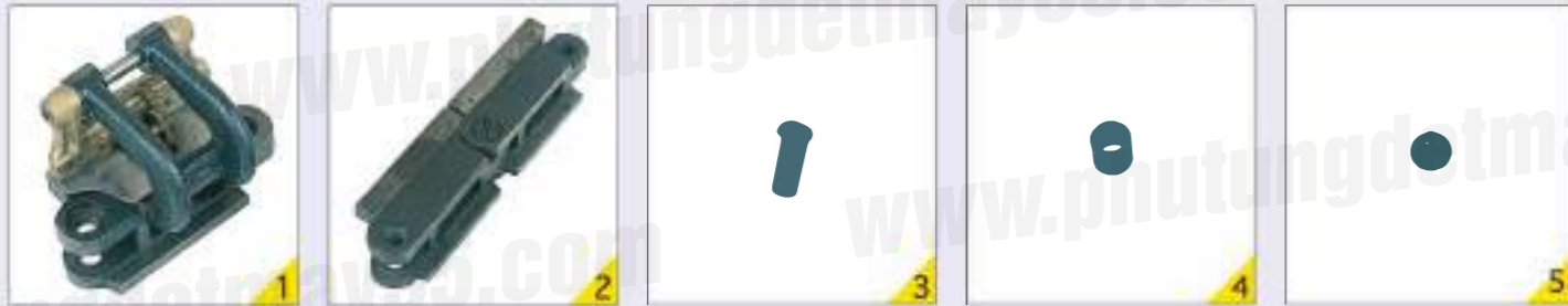
Clip, pin holder and chain Stenter brand: KCK Mercerizing Stentering Range
